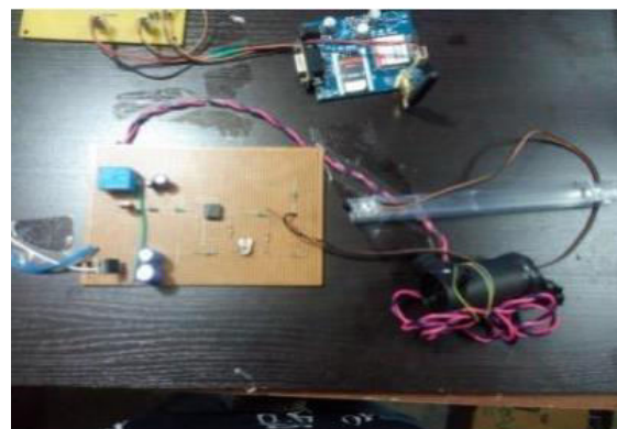
Fig.2. Sensor interfacing.
