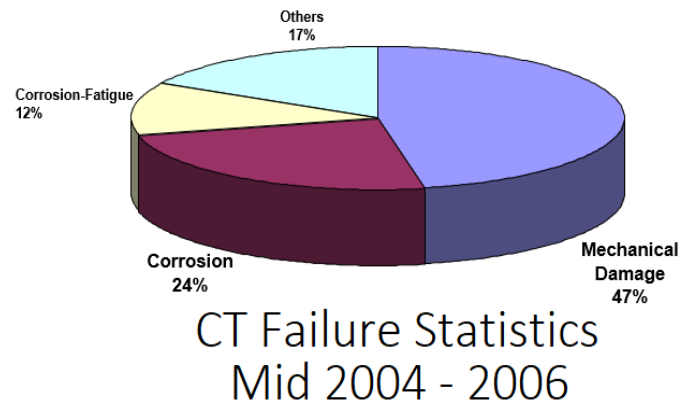
Figure 4. CT Failure Statistics Mid 2004 – 2006
