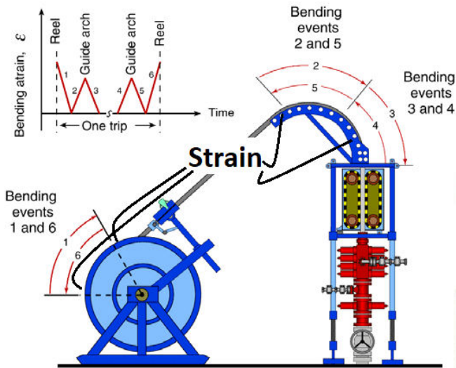
Figure 5. Failure due to Strain Effect
