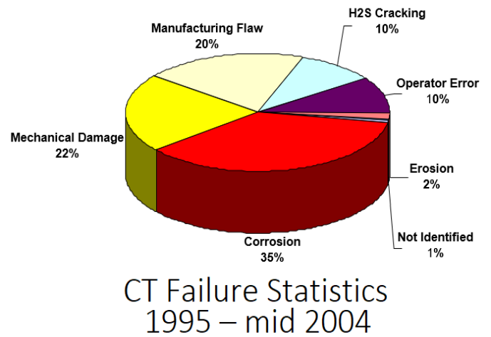
Figure 3. CT Failure Statistics 1995 – Mid 2004
