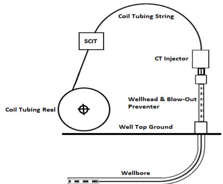
Figure 1. Overview of Well Vs. Coil Tubing Vs. SCIT Setup
