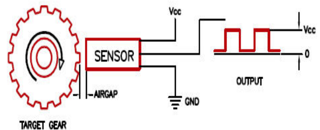
Figure 17. Non-Contact Magnetic Hall Sensor
