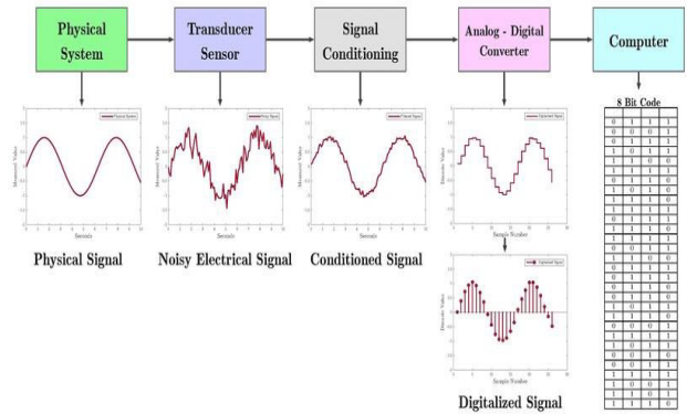
Figure 13. Digital Data Acquisition System
