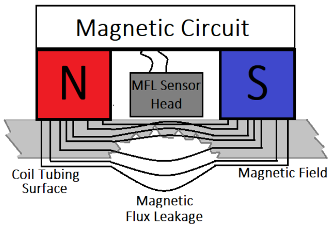
Figure 14. Magnetic Flux Leakage Principle
