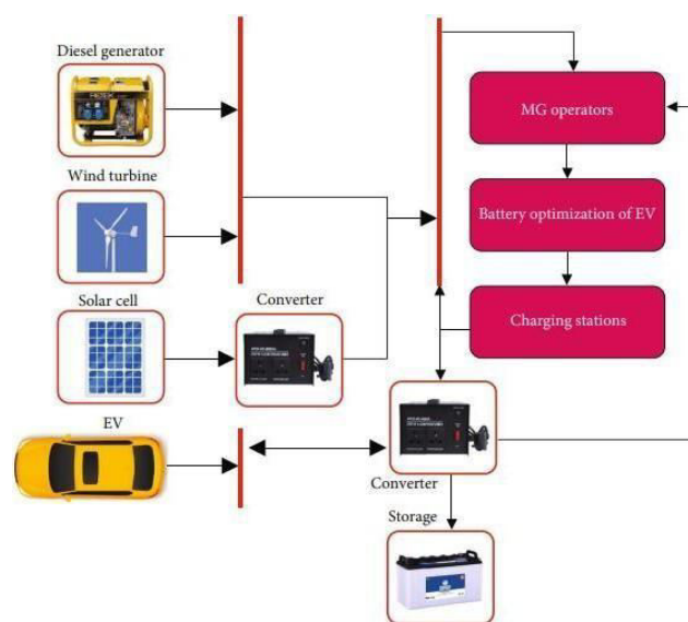
Fig: 2.1 Schematic diagram of the proposed multi-input inverter.
