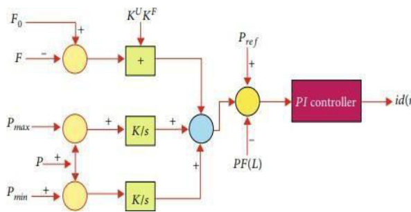
Figure 4: Block diagram of a droop control.
