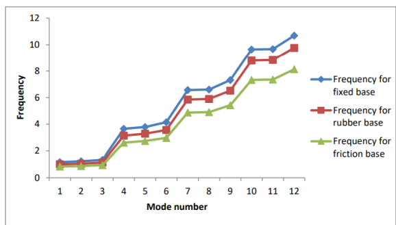
Comparison of frequency for different base conditions in Zone V
