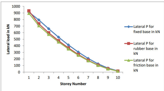
Comparison of Lateral load for different base conditions in Zone IV
