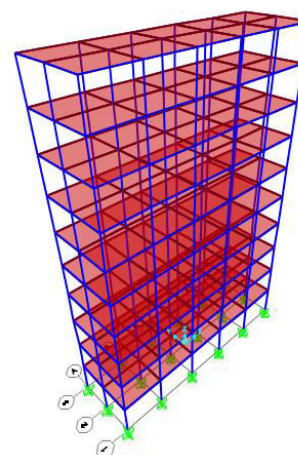
Building Model with friction isolator at supports
