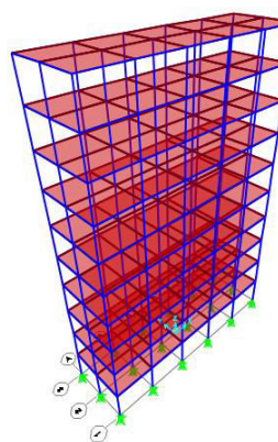
Building Model with rubber isolator at supports
