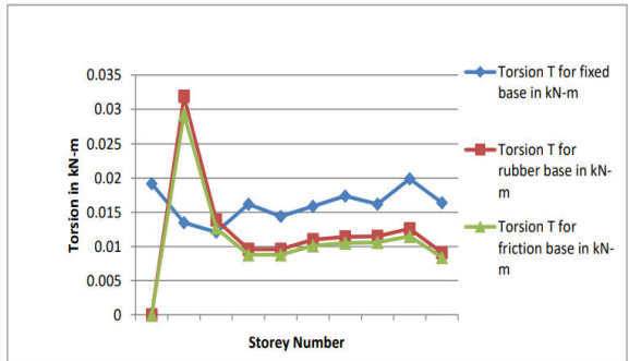
Comparison of Torsion T for different base conditions in Zone IV
