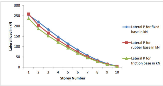
Comparison of Lateral load for different base conditions in Zone II
