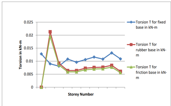
Comparison of Torsion T for different base conditions in Zone III
